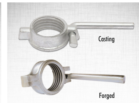
Prop Nut with Handle
