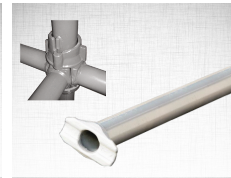
Ledgers (Cup lock System)
